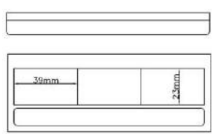
OK3 SIZE:L128mm*W49mm*H14mm
