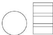
5F*3 SIZE: D30mm*H49mm
