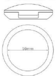
PH59-1 SIZE: D73mm*H22mm
