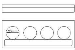
F4 SIZE:L128mm*W49mm*H14mm
