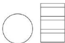
10F*3 SIZE: D37mm*H53mm
